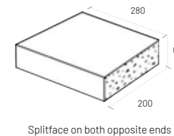
Coping Block J4
